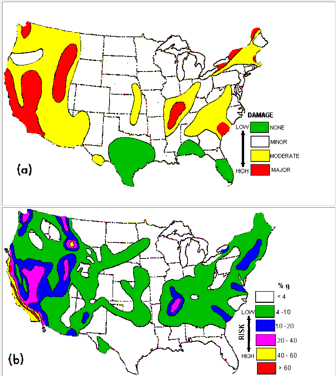
FIGURE 4. Earthquake risk maps of the United States: (a) Relative risk of damage, based to a large extent on known earthquake history (Algermissen, 1969).(b) Probabilistic risk map showing maximum horizontal ground acceleration with a 90-percent probability of not being exceeded in 50 years (Algermissen et al., 1982).
