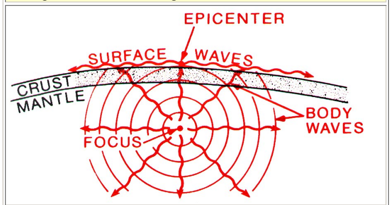
FIGURE 1. Highly generalized cross section of earth's crust and upper mantle depicting seismic waves, an earthquake focus and an epicenter.
