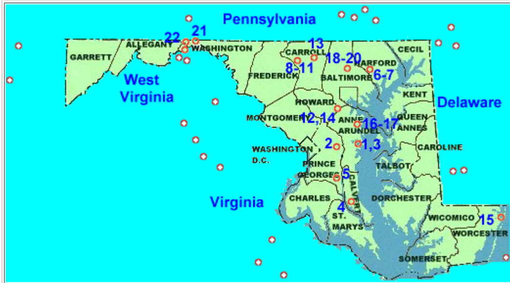
FIGURE 3. Map showing approximate epicenters of historic earthquakes in and near Maryland (from data in Stover et al., 1984; U.S. Geological Survey, 1990).
