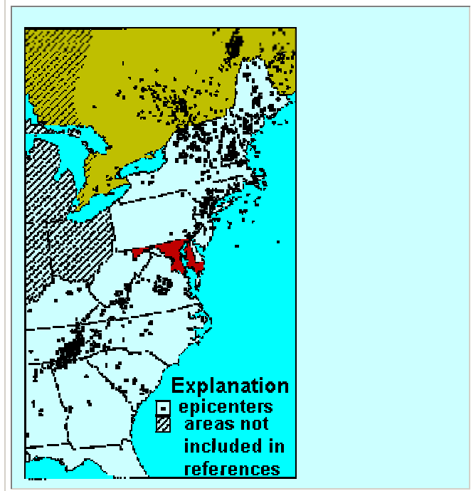
FIGURE 2. Earthquake epicenters in the eastern United States, 1976-1985 (from Foley et al., 1985; Sibol et al., 1985; and Stover et al., 1984).
